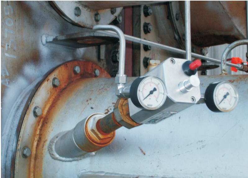
ACL 2000 installed on oil treater
